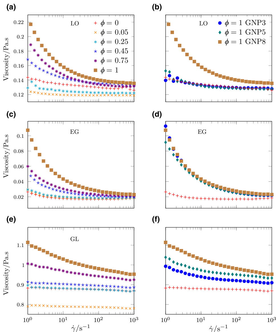
Fig. 12 Viscosity of LO+GNP, EG+GNP and GL+GNP solutions as a function of shear rate \dot{\gamma} , a, c, e for different \phi of GNP8 and b, d, f for different SSA at \phi = 1\% and 25\text{ }^\circ\text{C} (298.15 K)
