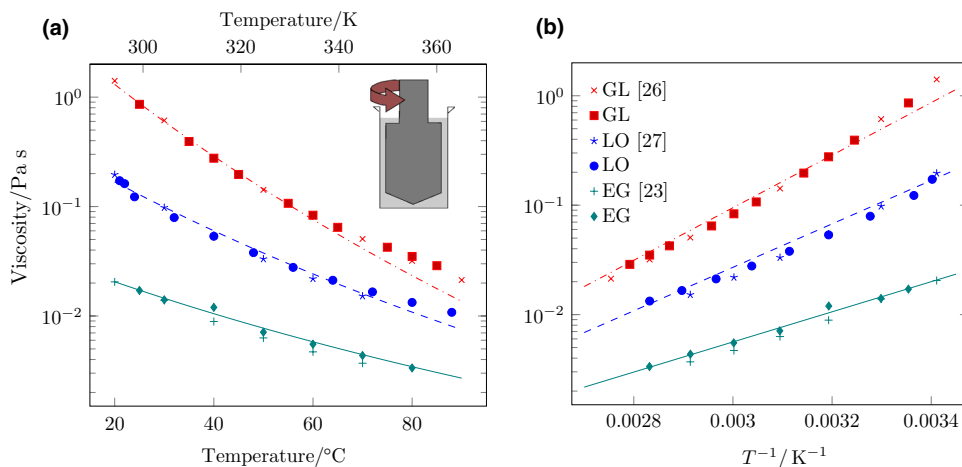
Fig. 4 Shear viscosity of EG, LO and GL as a function of a the temperature, T , and b 1/T . The lines represent Arrhenius fits: \eta(T) = A \exp(E_a/RT) presented in Table 2. The insert is a schematic of the concentric cylinder geometry
