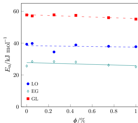
Fig. 11 Evolution of activation energy, E_a , as a function of the GNP8, \phi , for LO, EG and GL
