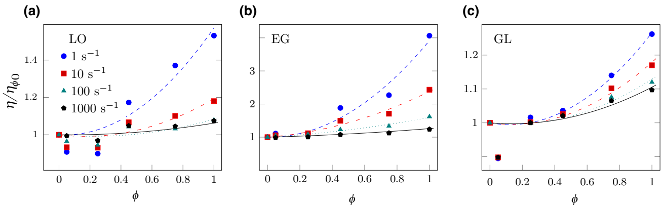
Fig. 13 Relative viscosity of a LO+GNP8, b EG+GNP8 and c GL+GNP8 as a function of the solid fraction at temperature 25 °C for different shear rates: 1 \leq \dot{\gamma} \leq 1000 \text{ s}^{-1} . The dashed lines correspond to the model (3) described in the text
